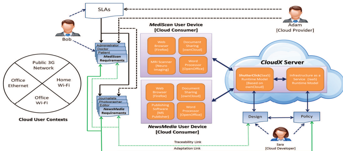
Figure 1. A Cloud Application Usage Scenario Diagram
